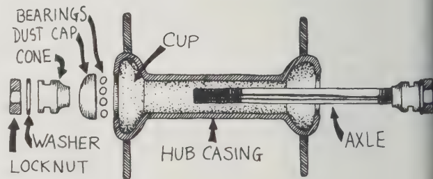
Hub, exploded view. —Anybody's Bicycle Book
